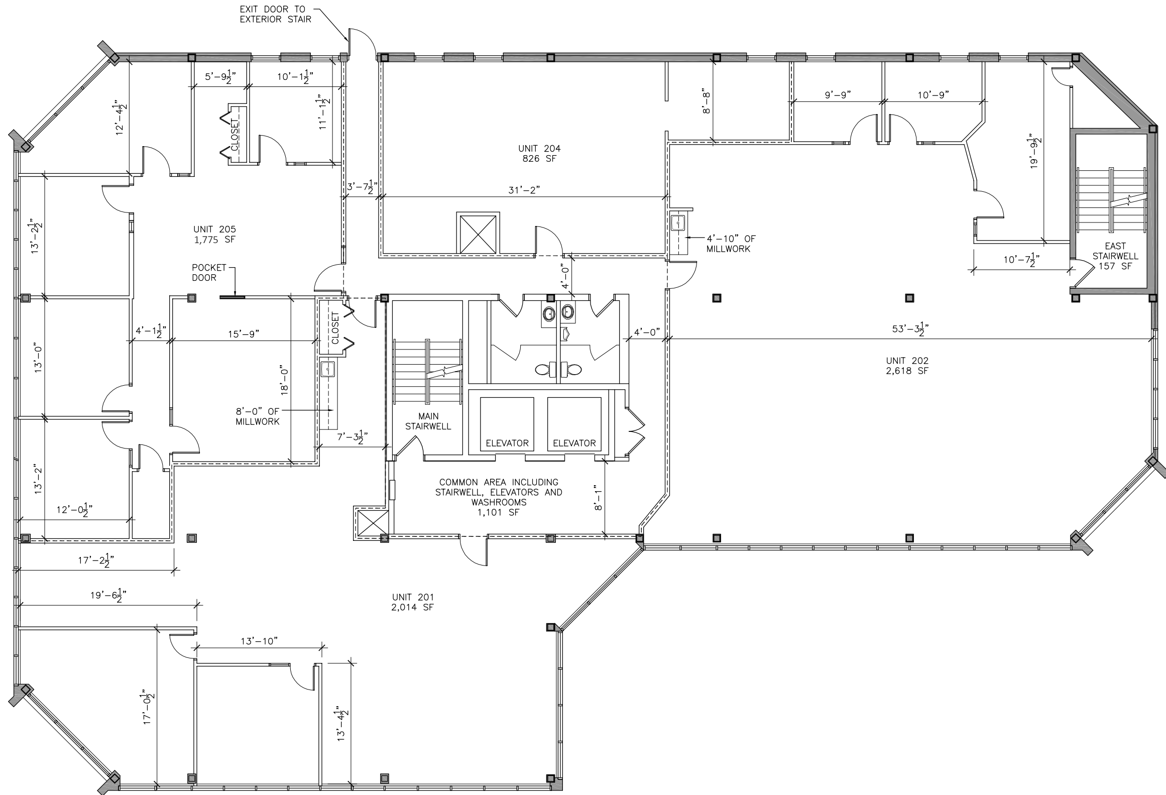
NORTH 1 SECOND FLOOR PLAN SCALE 1/8"=1'-0"
